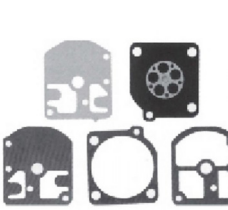
Kit reparo carburador stihl fs160/220/280/ fr220
